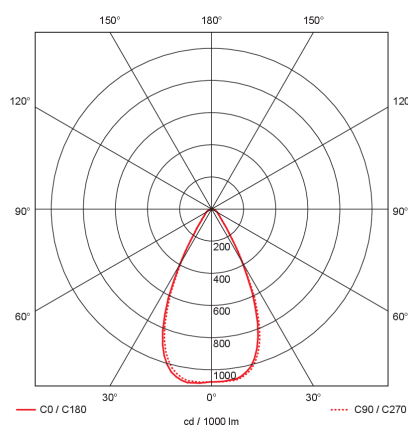
EXAIL 2131/P_T/ (160W - 19823 LM) (60° X 60°)
